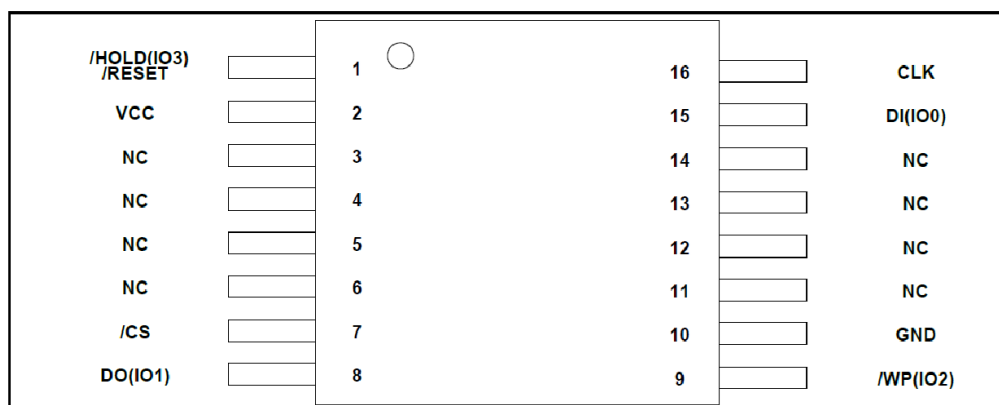
Figure 1b. 16-pin SOP 300-mil
