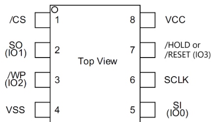
Figure 1a. 8-pin SOP 208-mil
