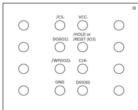
Figure 1d. DS25M4AE Pad Assignments, 16Ball WLCSP(Bottom View)
