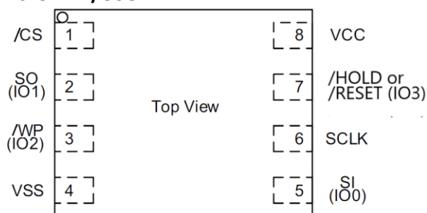
Figure 1c. 8-pad WSON 6x5-mm
