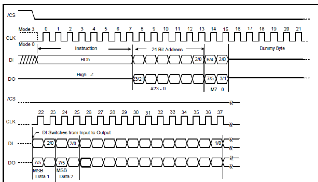
Figure18c. DTR Read Dual I/O Instruction (Previous instruction set M5-4 \neq 10, SPI Mode)
